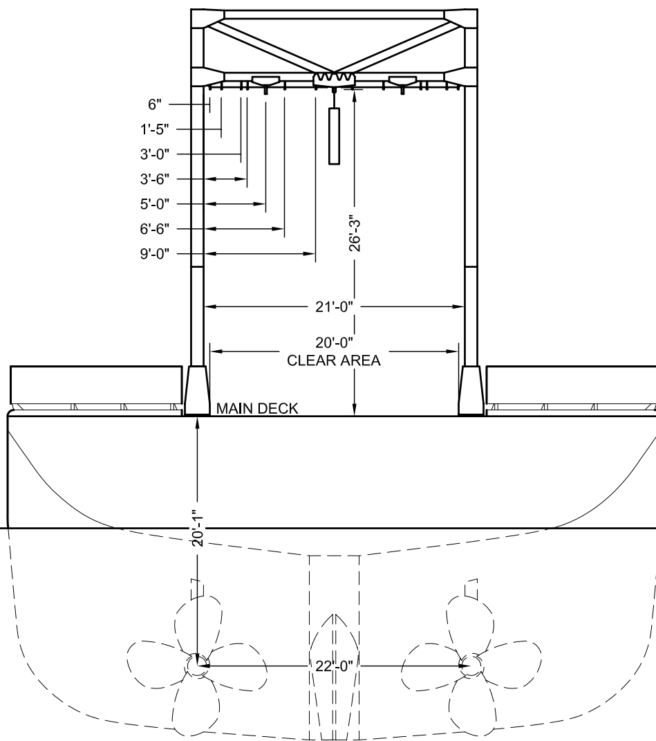
SECTION VIEW VERTICAL A-FRAME POSITION
