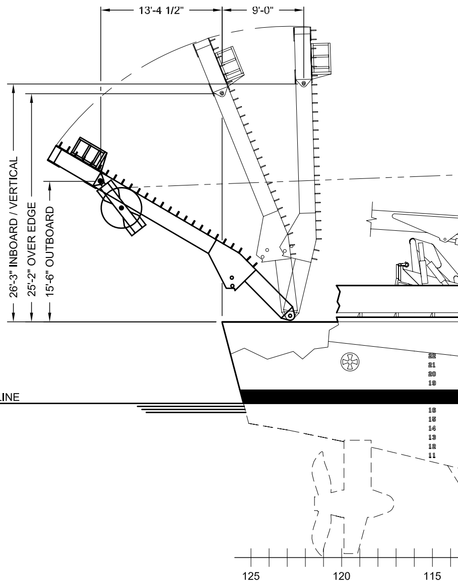
PROFILE VIEW INBOARD/OUTBOARD REACH
